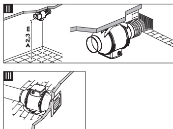
Multi-Point Exhaust System
