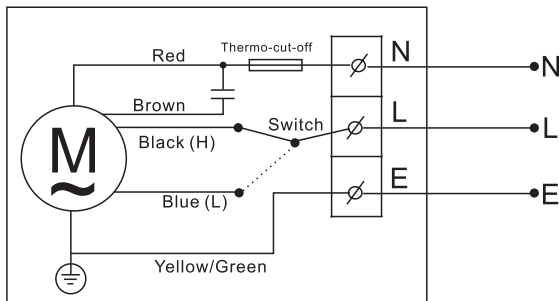
Figure 4. Electrical Wiring:
